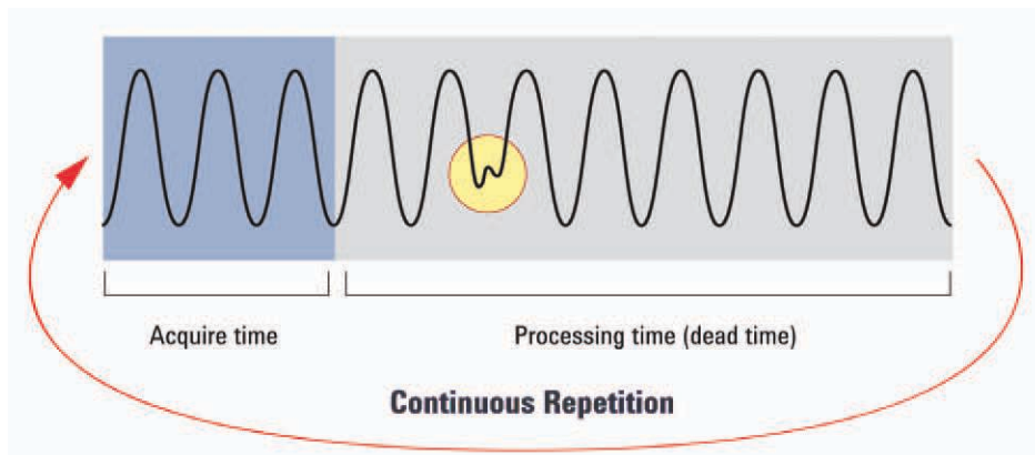
Figure 1: Oscilloscope dead time can hide rare events. A faster update rate (the inverse of dead time) can help increase your chances of seeing those infrequent events.
