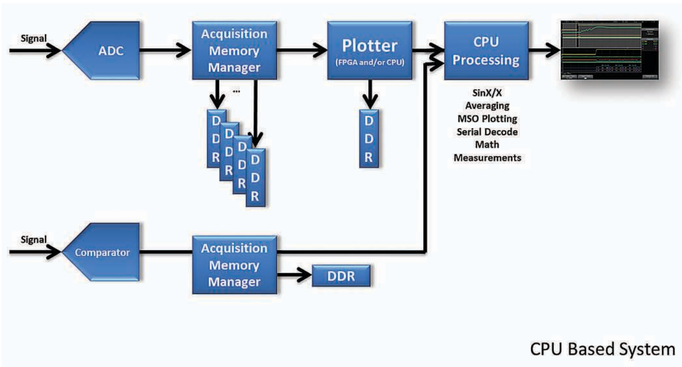
Figure 2: CPU-based Architecture Block Diagram showing how the CPU system is a bottle neck to overall waveform plotting.
