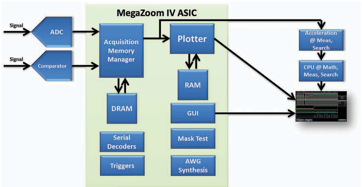
Figure 3: MegaZoom architecture with a custom ASIC driving the plotting of waveforms from acquisition memory.
